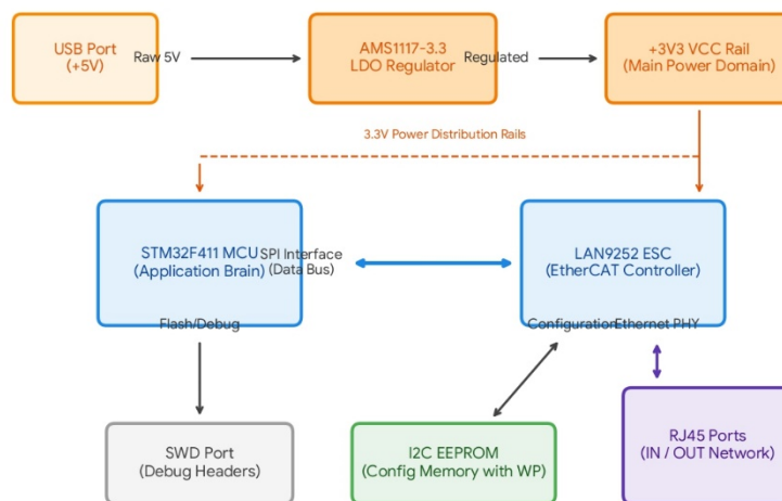
System Block Diagram: USB to EtherCAT Adapter Board V1.0
